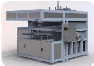
Single / double flip molding machine
